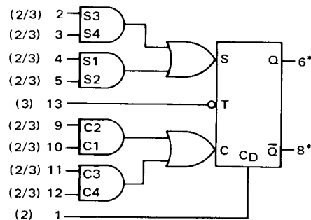
MC1815/MC1915 MC1816/MC1916 Parallel Gated Clocked Flip-Flop
