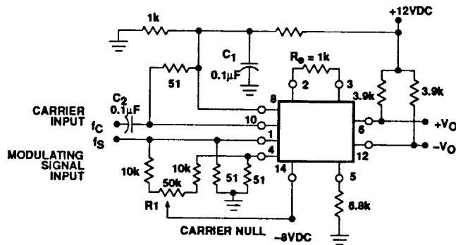
Carrier Rejection and Suppression
