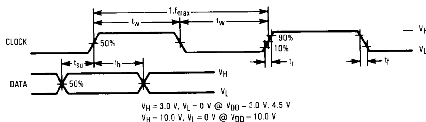
Figure 1. Switching Waveforms
