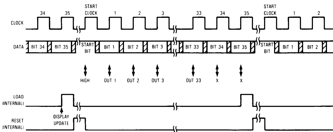
Figure 2. Timing Diagram
