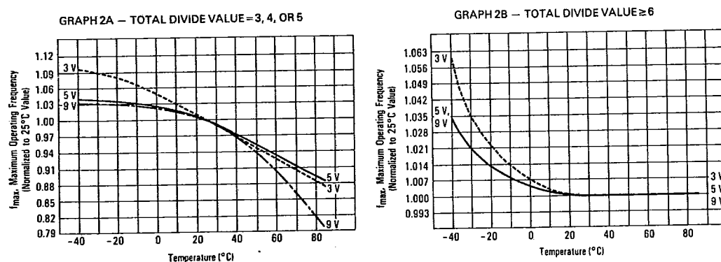
GRAPH 2 — f_{in} AND f_{osc} MAXIMUM FREQUENCY VERSUS TEMPERATURE FOR SINE AND SQUARE WAVE INPUTS
