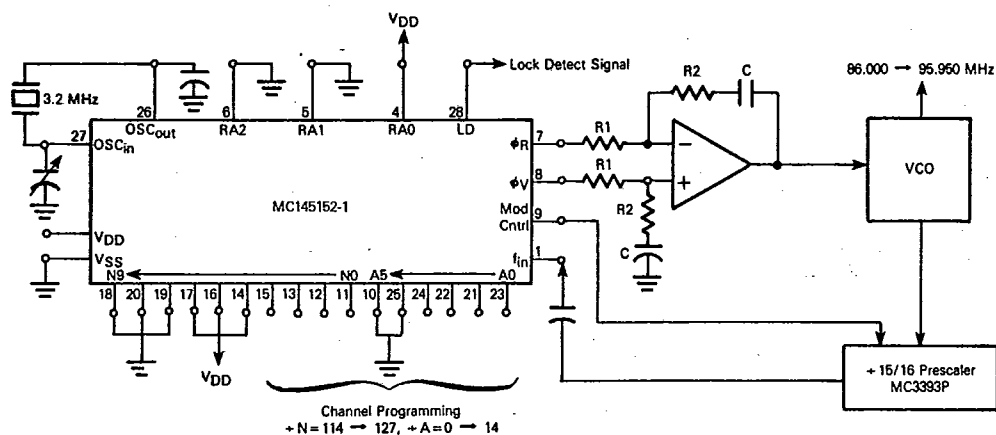
FIGURE 8 — AIRCRAFT NAV RECEIVER SYNTHESIZER DEMONSTRATES A LOW COST DUAL MODULUS SYSTEM EMPLOYING THE MC145152-1
