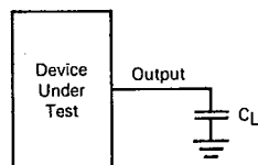
FIGURE 5 — TEST CIRCUIT
