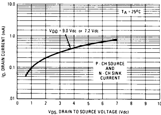
FIGURE 3 — TYPICAL COMPARATOR OUTPUT I-V CHARACTERISTIC
