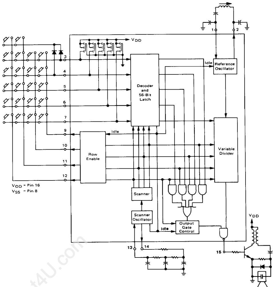
FIGURE 2 – TYPICAL APPLICATION
