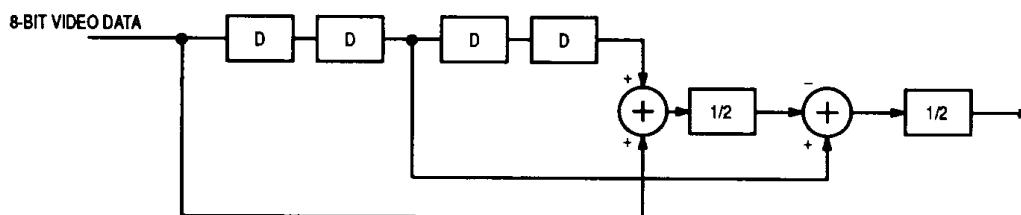
Figure 4. Horizontal Filter
