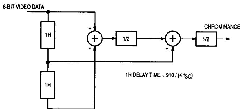
Figure 3. Vertical Filter
