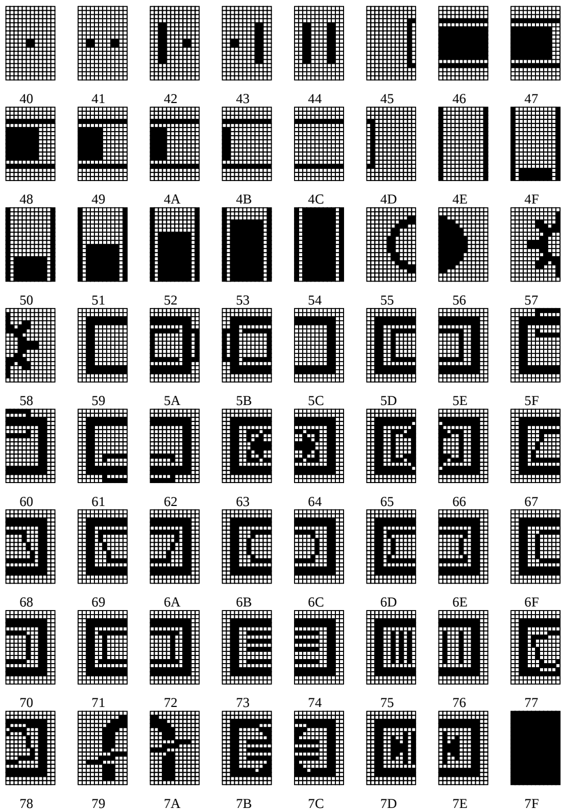
Figure 2. ROM contents for PAGE 0 ($40-$7F)
