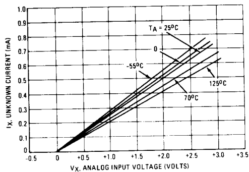
FIGURE 15 – UNKNOWN CURRENT versus ANALOG INPUT VOLTAGE
