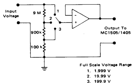
FIGURE 24 – DVM VOLTAGE RANGING
