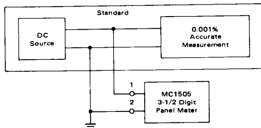
FIGURE 10 – CALIBRATION SET-UP
