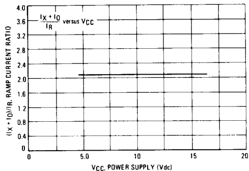
FIGURE 22 – RAMP CURRENT RATIO versus POWER SUPPLY
