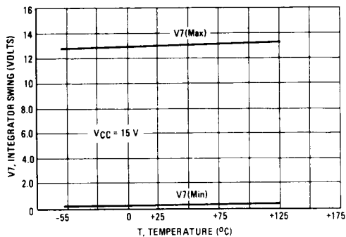
FIGURE 20 – INTEGRATOR OUTPUT SWING versus TEMPERATURE
