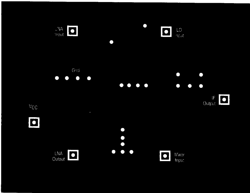
Figure 7. MC13141D1 Rev A – Ground Side View
