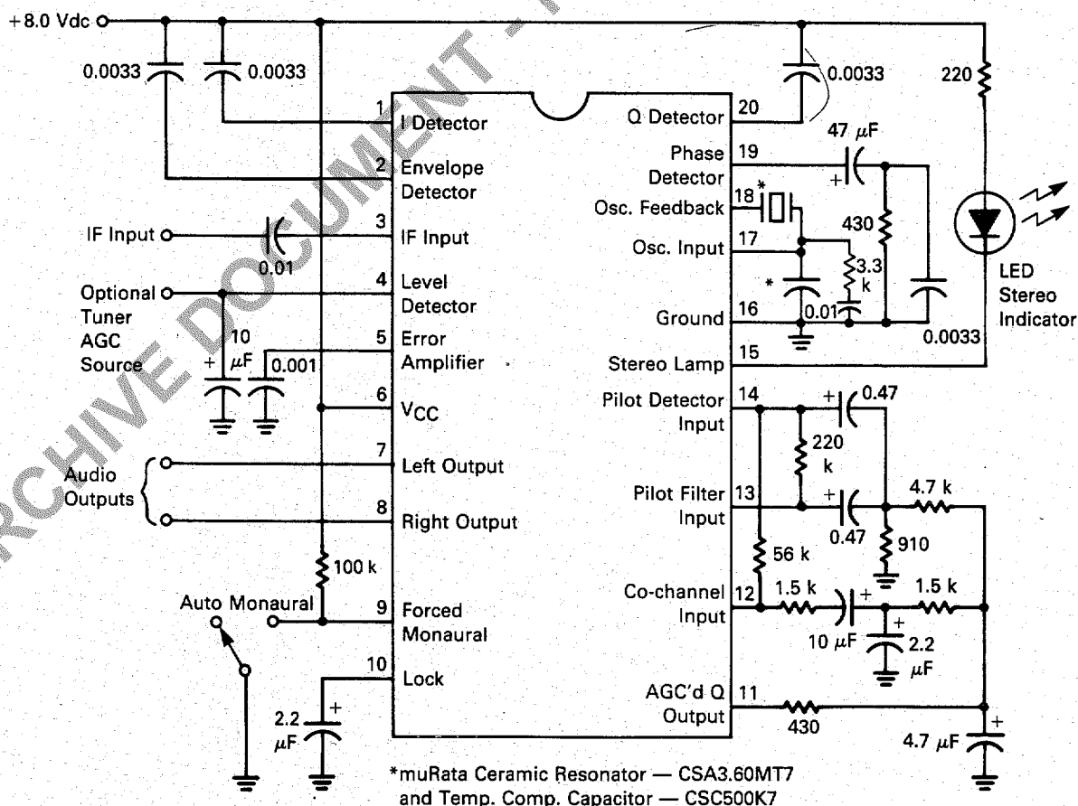
FIGURE 1 — TYPICAL APPLICATION
