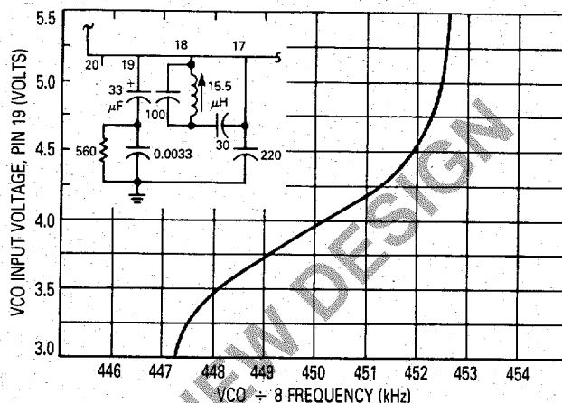
FIGURE 6 — L-C VCO
