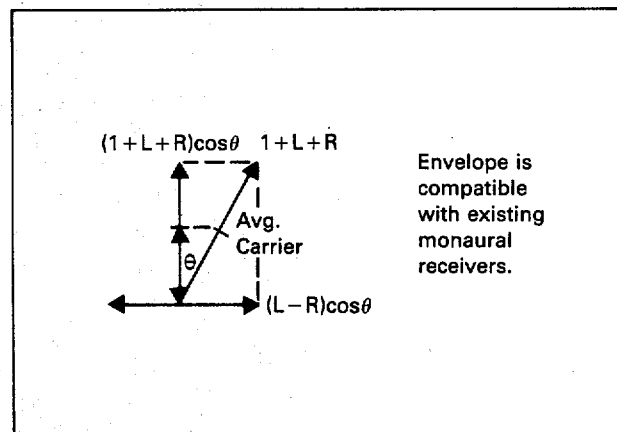
FIGURE 3 — MOTOROLA C-QUAM®
