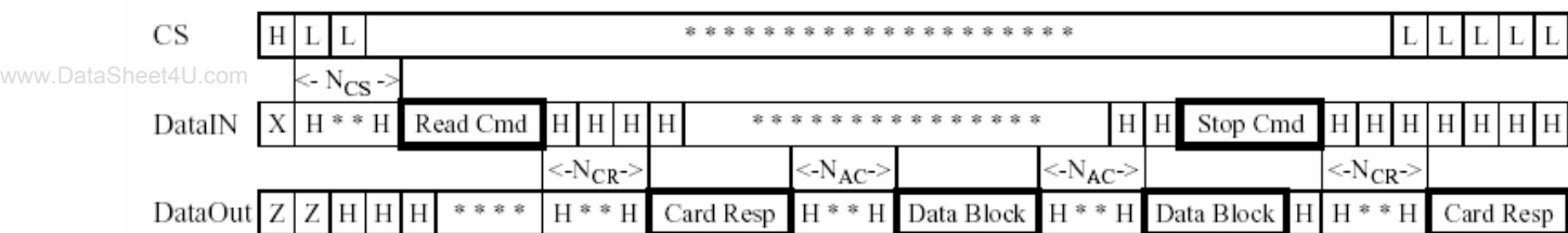
Figure 4-18 Timing diagram: Multiple block transaction, Stop transmission does not overlap data
