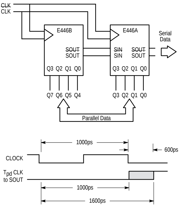
Figure 1. Cascaded 8:1 Converter Architecture
