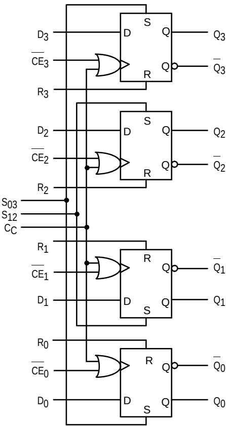
LOGIC DIAGRAM
