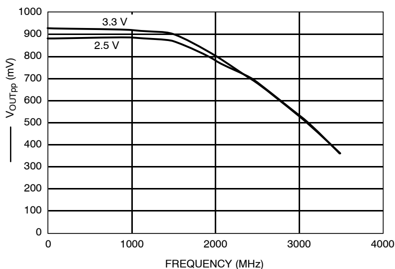
Figure 2. F_{\max} Typical
