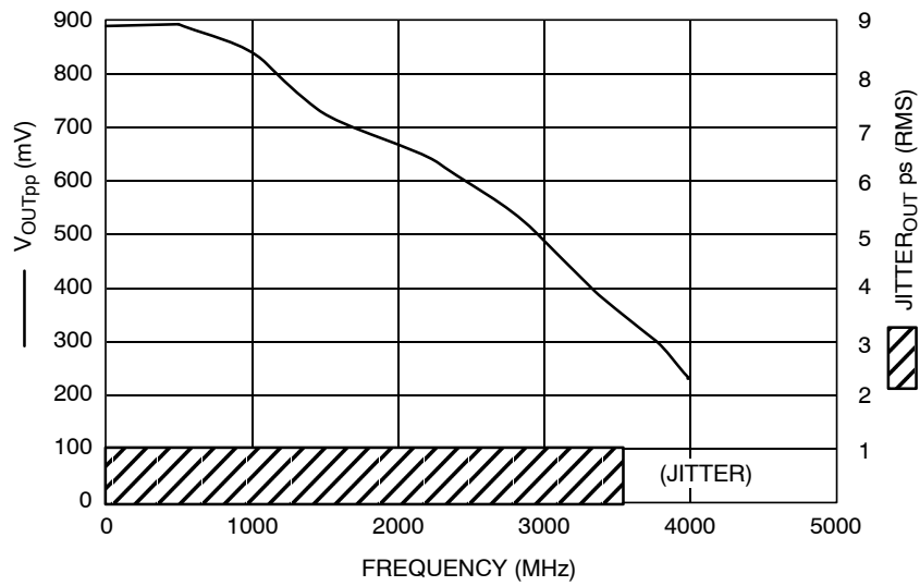
Figure 4. F_{max}/Jitter
