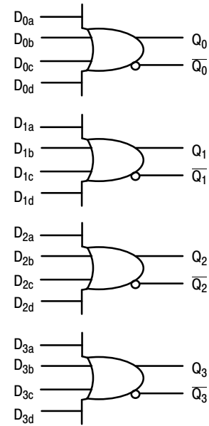
Figure 2. Logic Diagram
