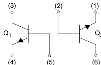
MBT3904DW1T1 STYLE 1
