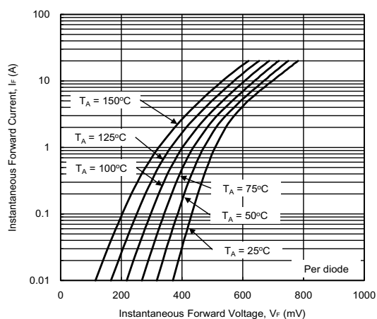
Fig. 1 - Forward Characteristics
