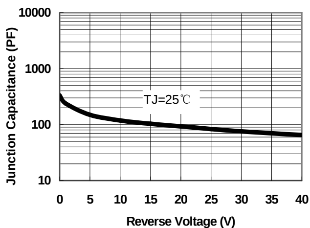
Fig.1-Typical Junction Capacitance
