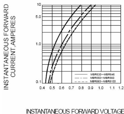
FIG.3 – TYPICAL INSTANTANEOUS FORWARD CHARACTERISTIC PER LEG
