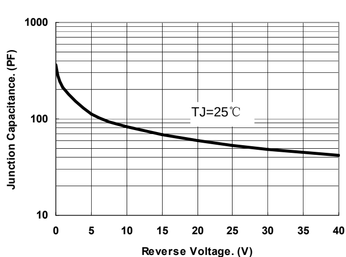
Fig.1-Typical Junction Capacitance
