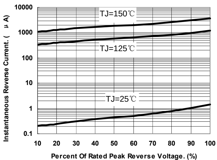
Fig.2-Typical Reverse Characteristics
