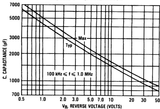
FIGURE 4 — CAPACITANCE
