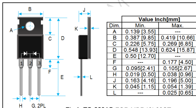
Fig 1. TO-220AB FOR MBR40L60CT
