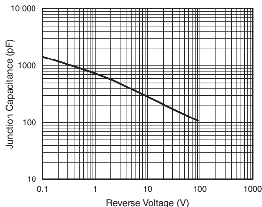
Fig. 4 - Typical Junction Capacitance Per Diode
