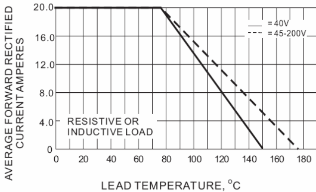
Fig.1 Forward current derating curve. For capacitive load derate by 20%
