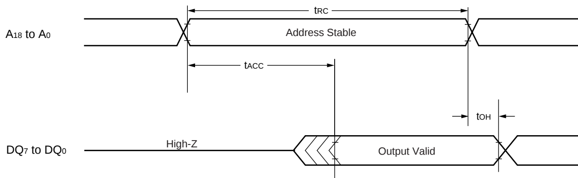
Figure 5.2 AC Waveforms for Read Operation
