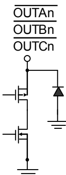
OUTAn,Bn,Cn terminal
