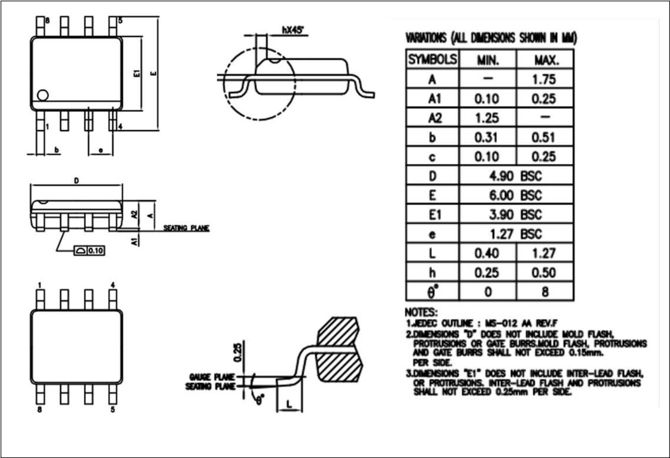
MBI5907GDT Outline Drawing
