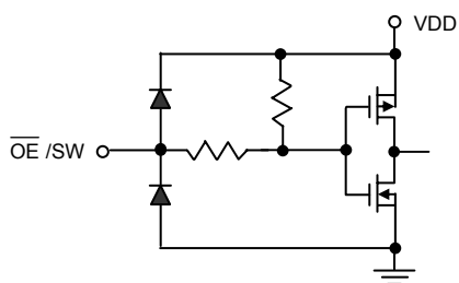
\overline{\text{OE}}/\text{SW} Terminal
