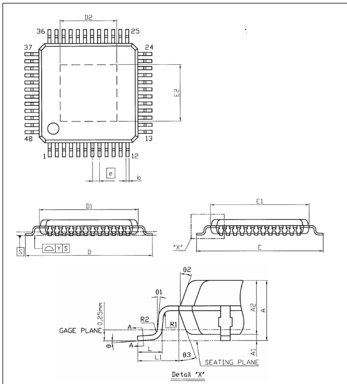
MBI5368 GLQ Outline Drawing
