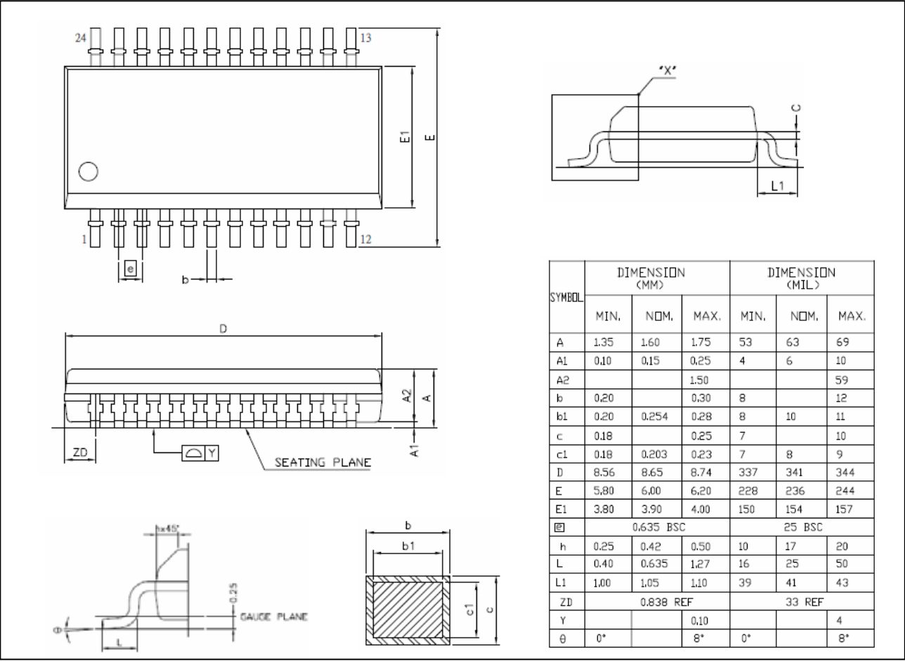
MBI5026GP\GPA Outline Drawing
