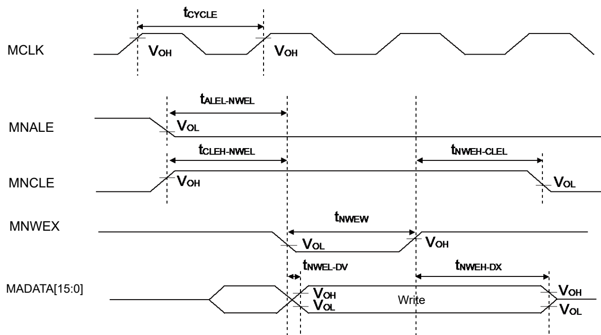
NAND Flash Memory Command Write
