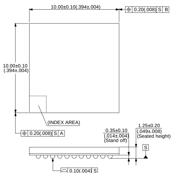
112-ball plastic PFBGA (BGA-112P-M04)
