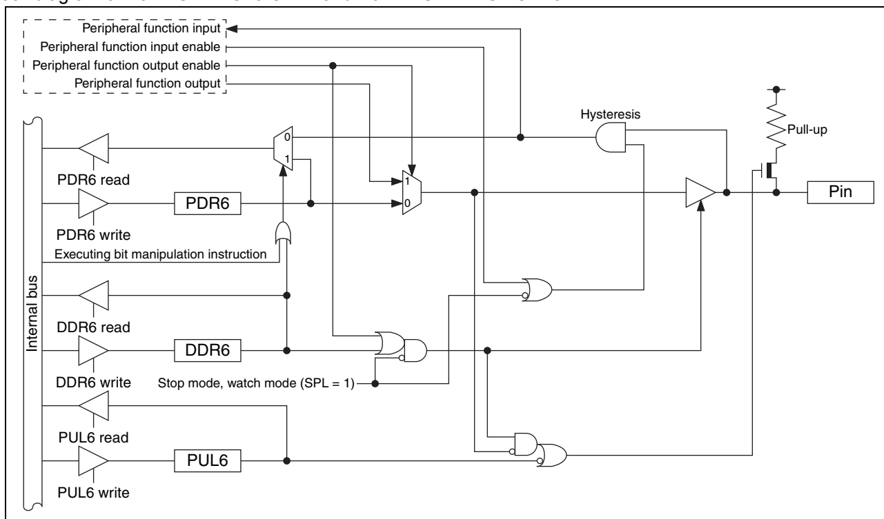
• Block diagram of P64/EC1/PPG10/OPT2 and P67/PPG21/TRG1/OPT5
