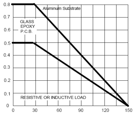
FIG.1 -- DERATING CURVE FOR OUTPUT RECTIFIED CURRENT
