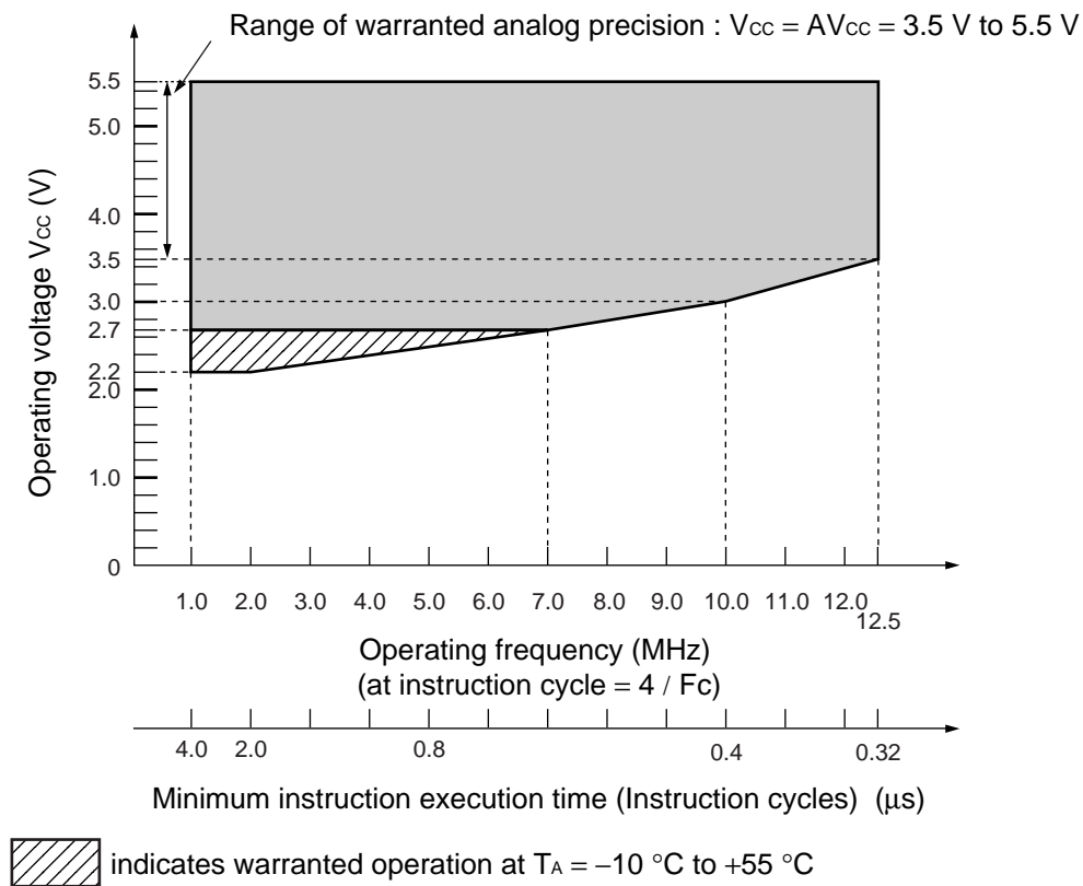
Operating voltage vs. operating frequency (MB89P538/MB89PV530)
