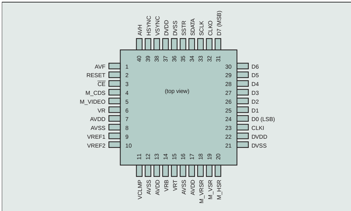
Figure 2. MB86S01 Pin Assignments
