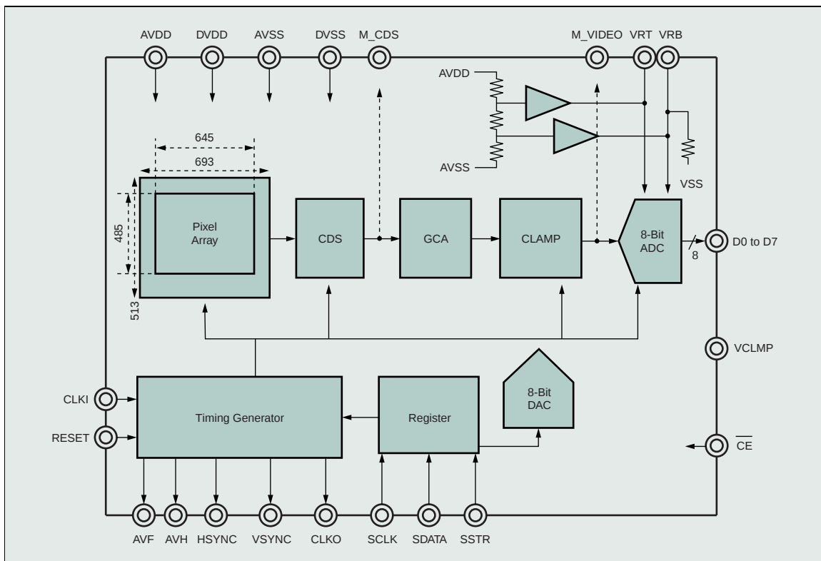
Figure 3. MB86S01 Block Diagram
