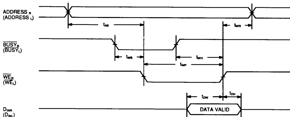
CONTENTION WRITE CYCLE No. 1 *1 *2 *3 ( \overline{WE} CONTROLLED)
