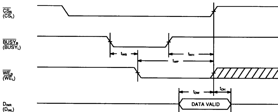
CONTENTION WRITE CYCLE No. 2 *3 : *1 *2 *3 ( \overline{CS} CONTROLLED)
