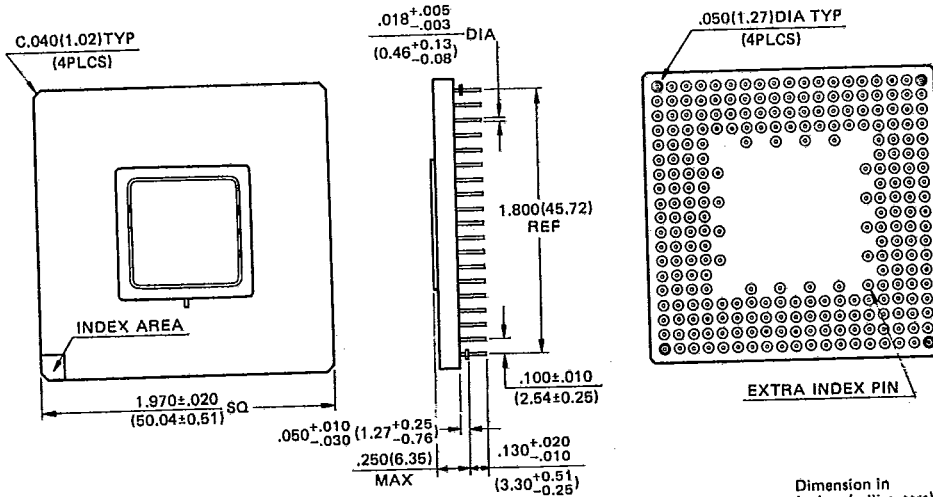
256-LEAD CERAMIC (METAL SEAL) PIN GRID ARRAY PACKAGE (CASE No.: PGA-256C-A03)
