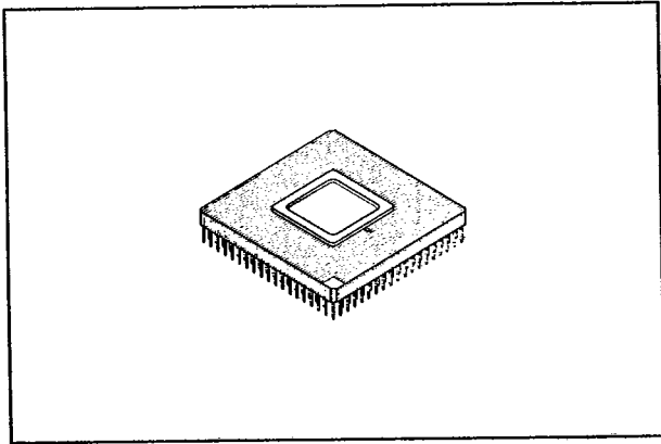
256-LEAD CERAMIC (METAL SEAL) PIN GRID ARRAY PACKAGE (CASE No.: PGA-256C-A03)
