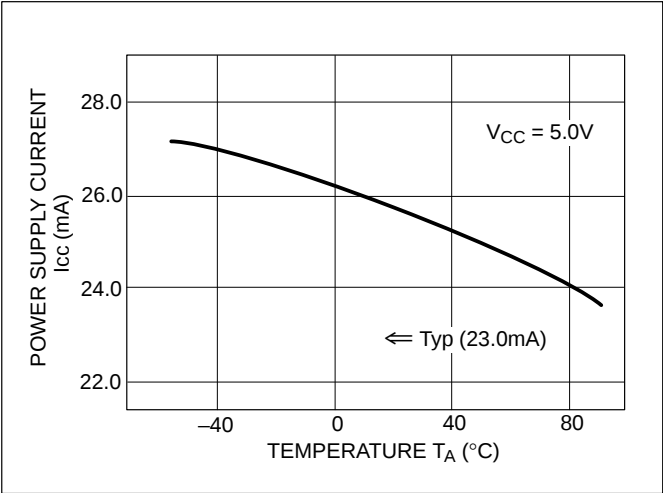
Figure 10. Power Supply Current vs. Temperature
