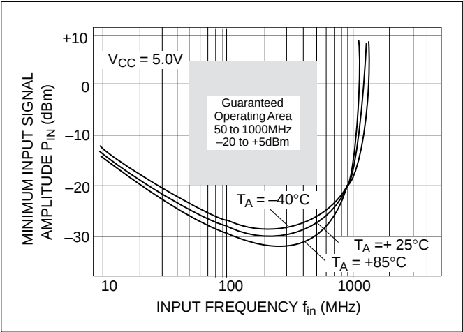
Figure 6. Input Sensitivity Curve (1/2 Divide Ratio) Temperature Dependency
