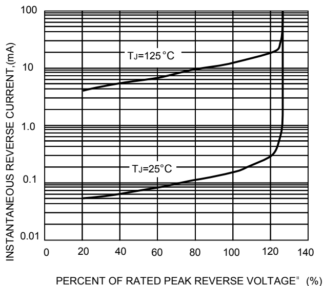
FIG.3-TYPICAL REVERSE CHARACTERISTICS
