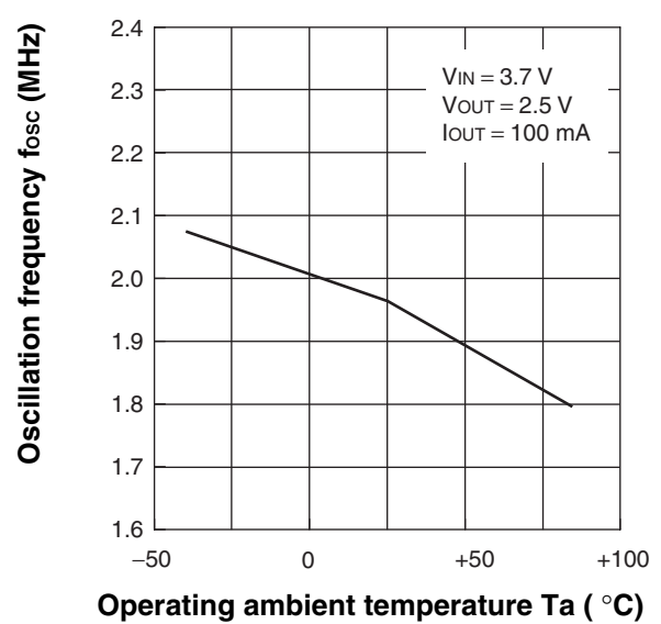
Oscillation frequency vs. Operating ambient temperature
