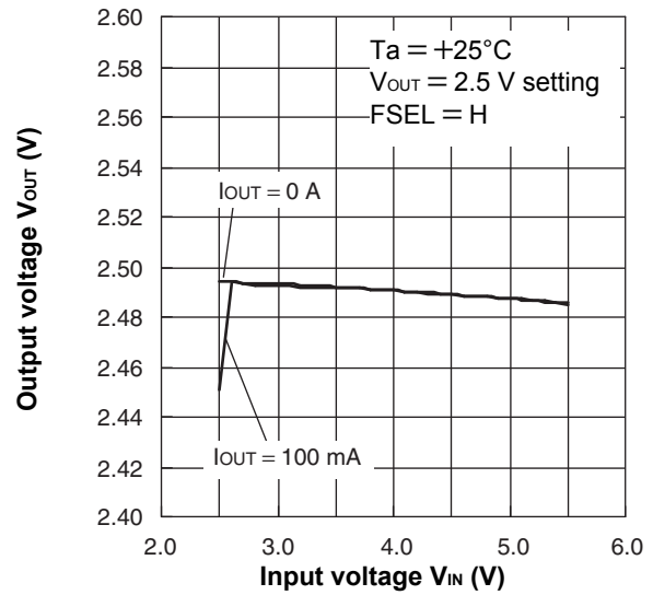
Output voltage vs. Input voltage (3.2 MHz)
