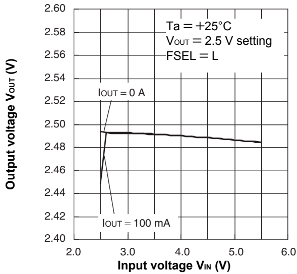
Output voltage vs. Input voltage (2.0 MHz)
