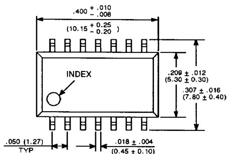
14-LEAD PLASTIC FLAT PACKAGE (CASE No.: FPT-14P-M01)
