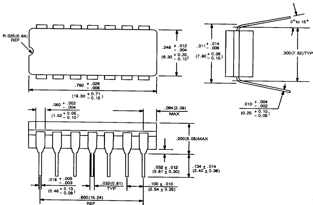
14-LEAD CERAMIC (CERDIP) DUAL-IN-LINE PACKAGE (CASE NO.: DIP-14C-CO1)
