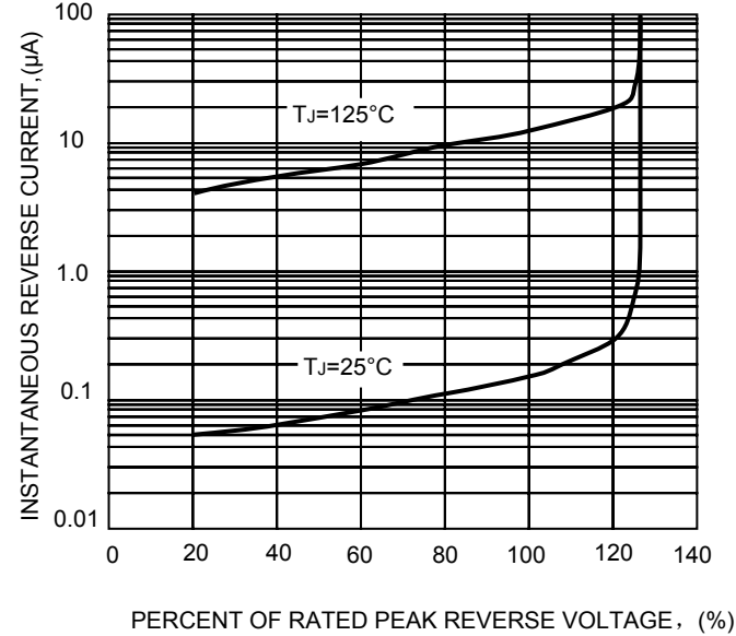
FIG.3-TYPICAL REVERSE CHARACTERISTICS
