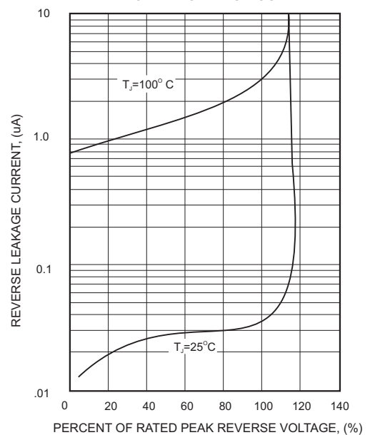
FIG.4-TYPICAL REVERSE CHARACTERISTICS
