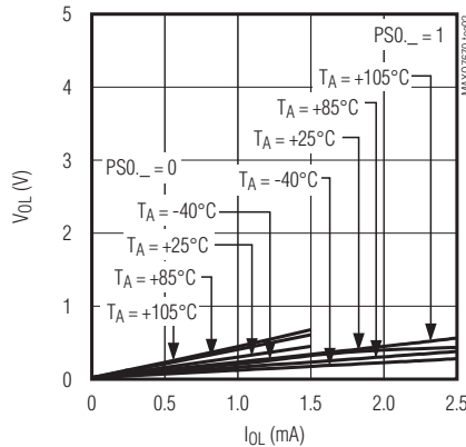
GPO_ OUTPUT LOW VOLTAGE vs. SINK CURRENT
