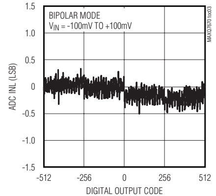
ADC INL vs. CODE (REF ADC = +3.3V, 150.9ksps, PGA GAIN = 16V/V)
