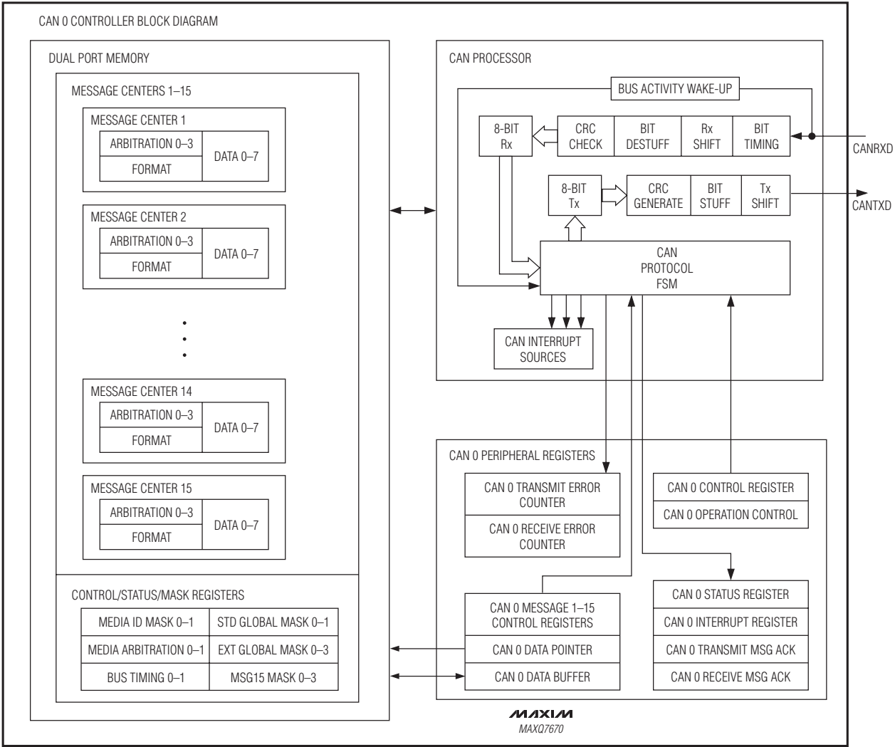
Figure 9. CAN 0 Controller Block Diagram
