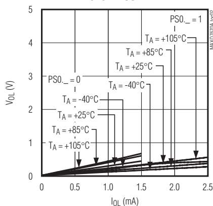
GPO 1 OUTPUT LOW VOLTAGE vs. SINK CURRENT
