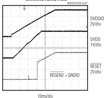
DVDD, RESET POWER-UP CHARACTERISTICS
