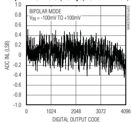
ADC INL vs. CODE (REF ADC = +3.3V, 75ksps, PGA GAIN = 16V/V)
