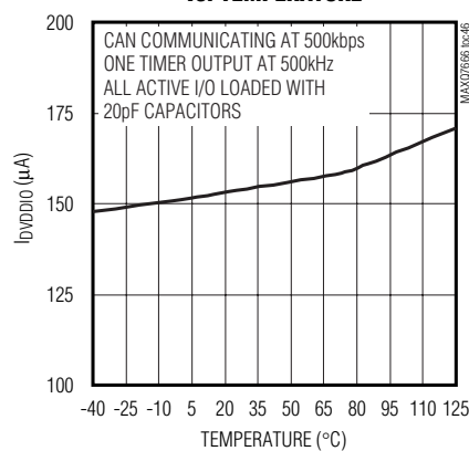
DV_{DDIO} DYNAMIC SUPPLY CURRENT vs. TEMPERATURE
