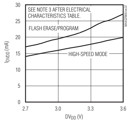
DV_{DD} ACTIVE SUPPLY CURRENT vs. DV_{DD} SUPPLY VOLTAGE
