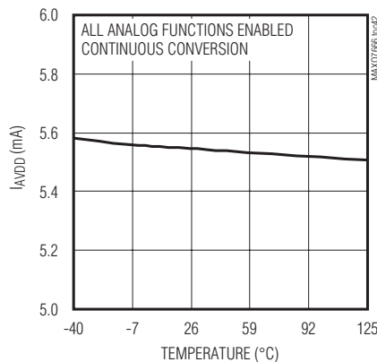
AV_{DD} ACTIVE SUPPLY CURRENT vs. TEMPERATURE
