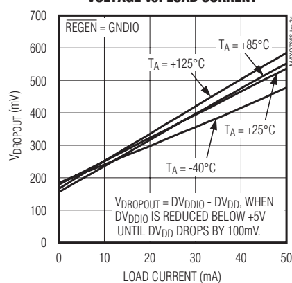
DV DD LINEAR REGULATOR DROPOUT VOLTAGE vs. LOAD CURRENT
