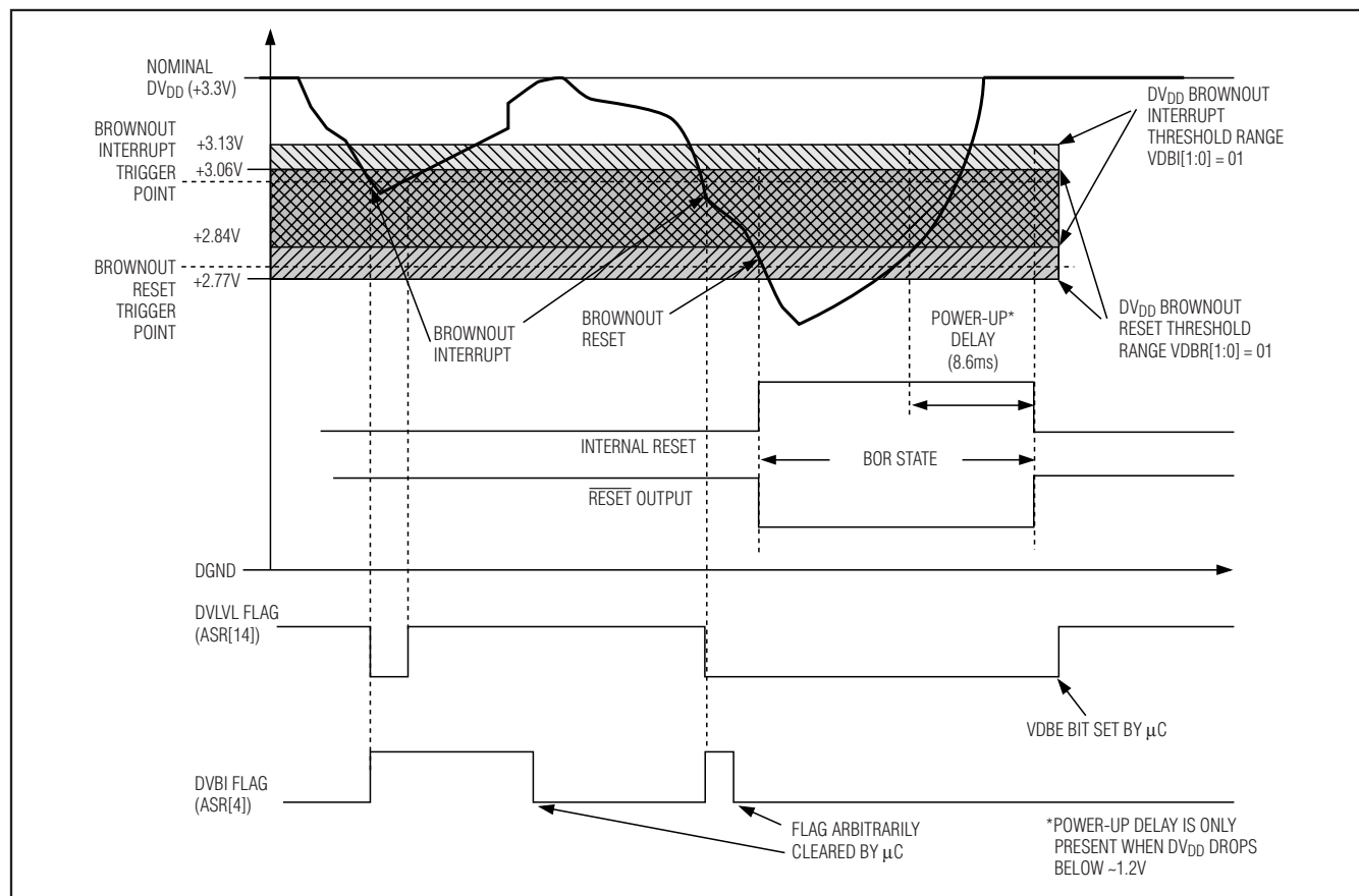
Figure 5. DVDD Brownout Interrupt Detection
