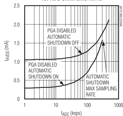
AV_{DD} SUPPLY CURRENT vs. ADC SAMPLING RATE
