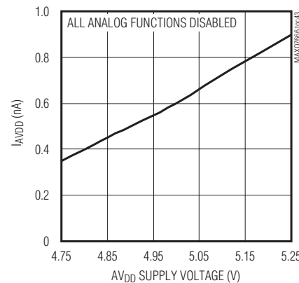
AV_{DD} SHUTDOWN SUPPLY CURRENT vs. AV_{DD} SUPPLY VOLTAGE
