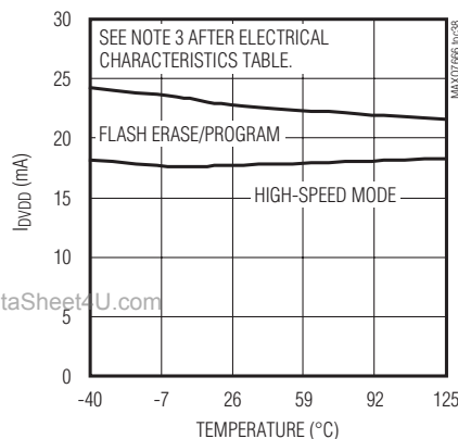
DV_{DD} ACTIVE SUPPLY CURRENT vs. TEMPERATURE
