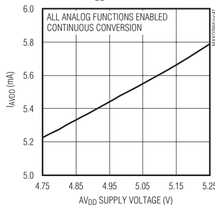
AV_{DD} ACTIVE SUPPLY CURRENT vs. AV_{DD} SUPPLY VOLTAGE
