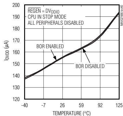
DV_{DD} STOP-MODE SUPPLY CURRENT vs. TEMPERATURE
