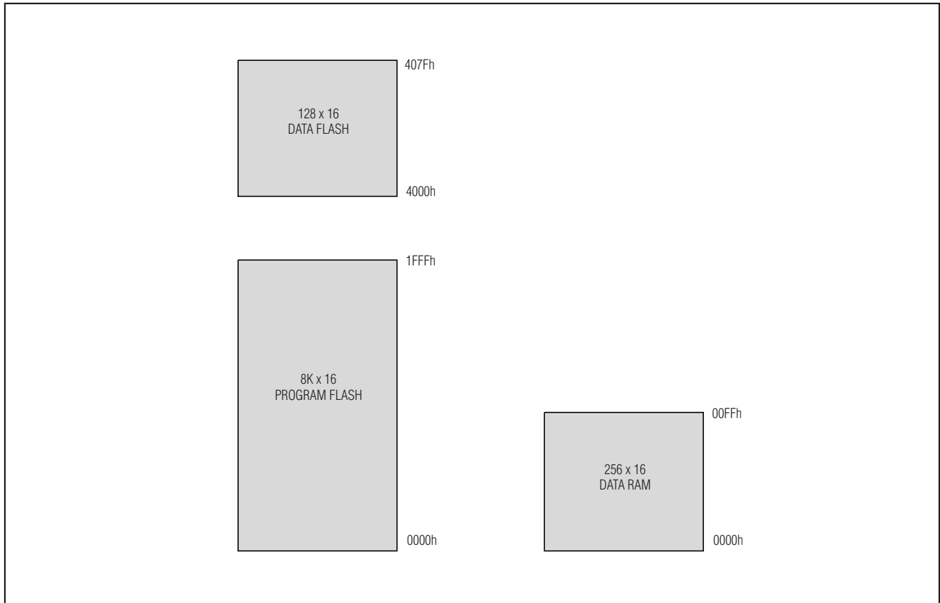
Figure 15. Memory Organization
