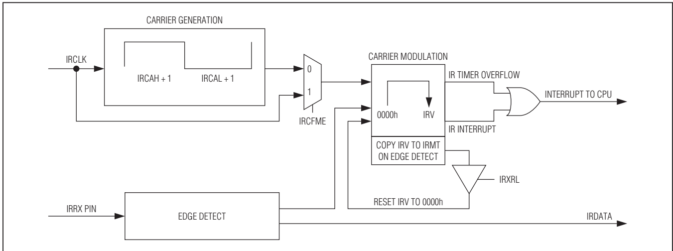
Figure 5. IR Capture
