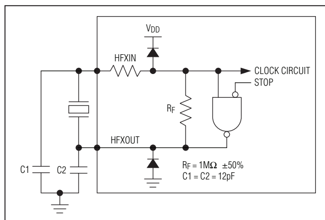
Figure 9. On-Chip Oscillator
